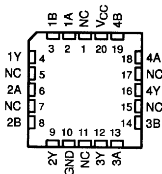
SN54ALS86, SN54AS86A . . . FK PACKAGE (TOP VIEW)
