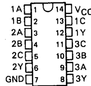
SN54ALS10A, SN54AS10 . . . J PACKAGE SN74ALS10A, SN74AS10 . . . D OR N PACKAGE
