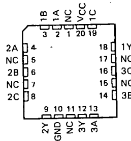
SN54ALS10A, SN54AS10 . . . FK PACKAGE
