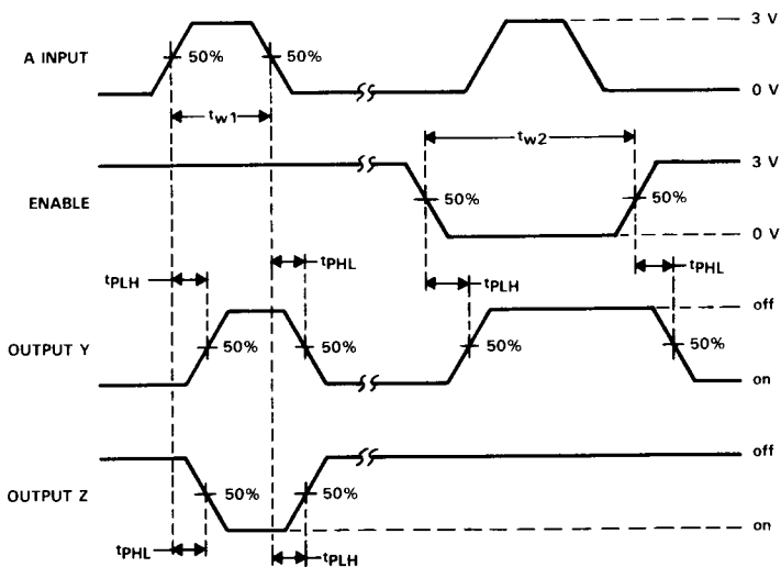
VOLTAGE WAVEFORMS
