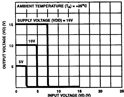
FIGURE 7. TYPICAL VOLTAGE TRANSFER CHARACTERISTICS
