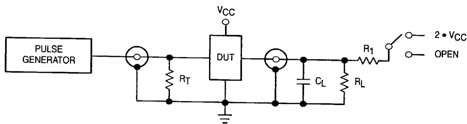
Figure 1. AC Waveforms
