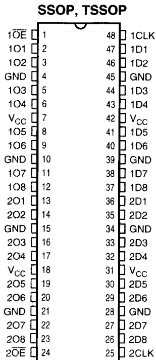
Figure 2. Pin Configuration (All Pins Top View)
