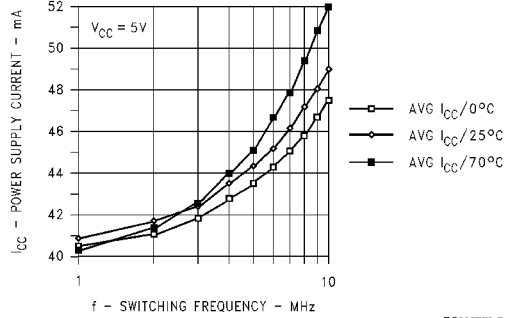
DS26LS31CN Unloaded I_{CC} vs Frequency vs T_A
