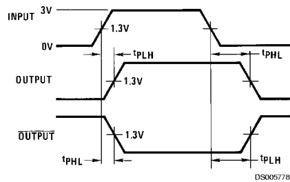
FIGURE 2. Propagation Delays
