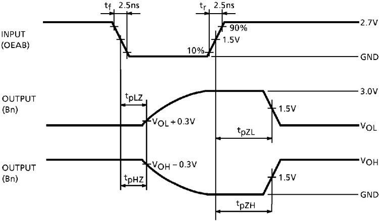
Fig.4 t_{pLZ} , t_{pHZ} , t_{pZL} , t_{pZH}
