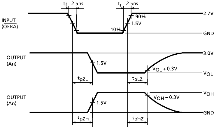
Fig.3 t_{pLZ} , t_{pHZ} , t_{pZL} , t_{pZH}
