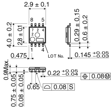
BU7242FVM (MSOP8) (Unit : [mm])
