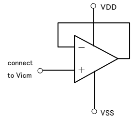
Fig.1 The example of disabled circuit
