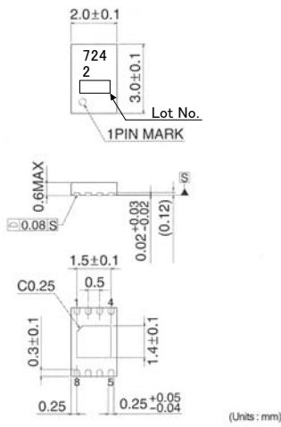
BU7242NUX (VSON008X2030) (Unit : [mm])
