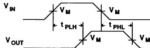
Waveform 2. For Non-Inverting Outputs
