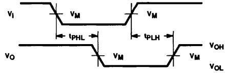
Waveform 2. Waveform for Non-Inverting Outputs
