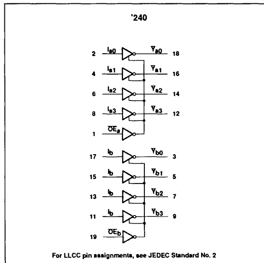
LOGIC SYMBOL
