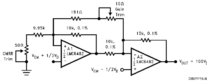
FIGURE 16. Low-Power Two-Op-Amp Instrumentation Amplifier
