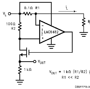
FIGURE 22. Positive Supply Current Sense
