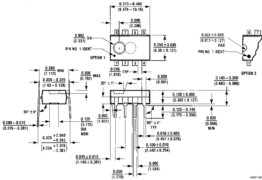
8-Pin Molded Dual-In-Line Package Order Package Number LMC6482AIN, LMC6482IN or LMC6482MN NS Package Number N08E
