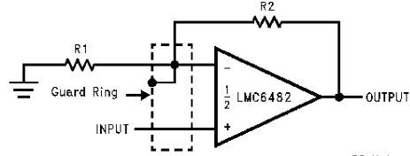
Non-Inverting Amplifier
