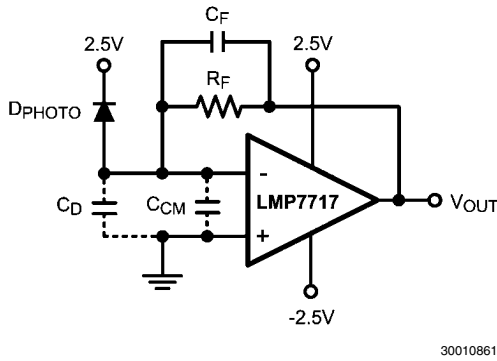
FIGURE 16. Transimpedance Amplifier
