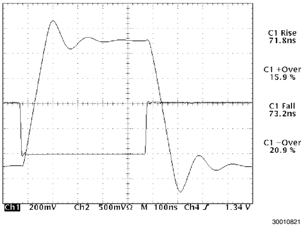
FIGURE 10. LMP7715 Response
