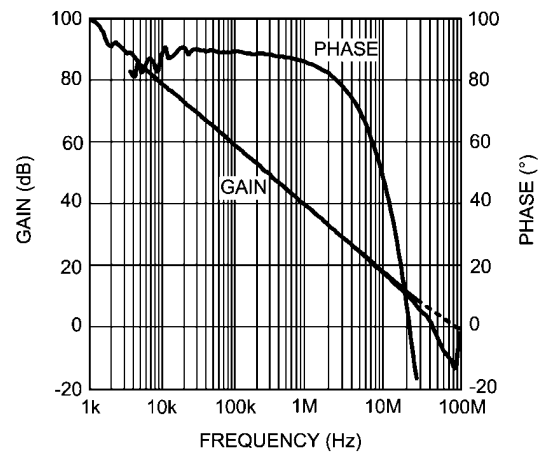
FIGURE 1. LMP7717 A_{VOL} vs. Frequency
