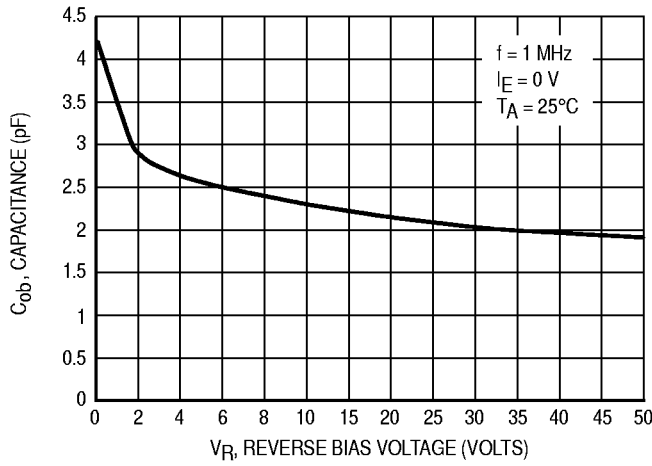
Figure 39. Output Capacitance
