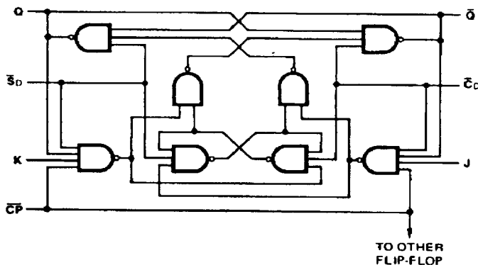
LÓGIC DIAGRAMS (one half shown) '76, 'H76
