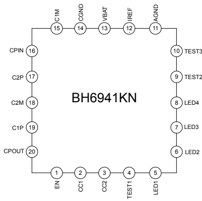
Fig.21 Pin Location Diagram (BH6941KN TOP View)
