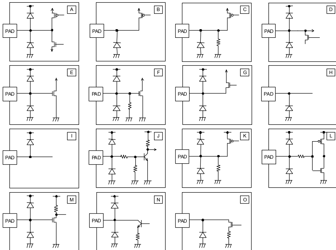
Fig.27 Pin Diagram
