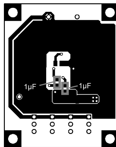
Fig.29 Example of BH6943KN Layout Pattern (Rear, Top View)
