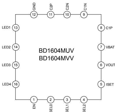
Fig.25 Pin Location Diagram (BD1604MUV/MVV Top View)
