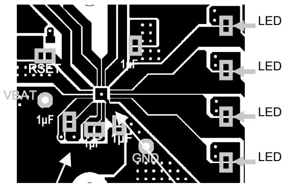
The GND pin and Cin must be placed nearby.
