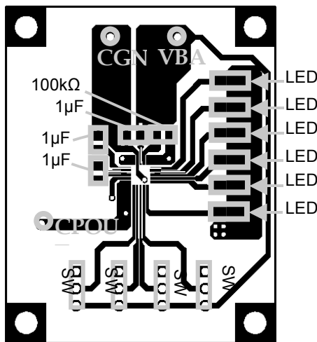
Fig.28 Example of BH6943KN Layout Pattern (Front, Top View)
