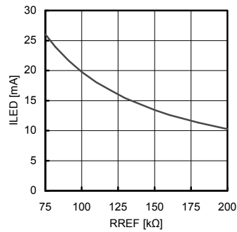
Fig.8 LED LED Output Current vs. R REF (BH6943KN)
