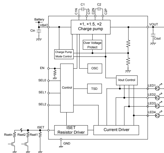
Fig.35 Controlling the Current in the BD1604MUV/MVV by Changing the Resistance Value
