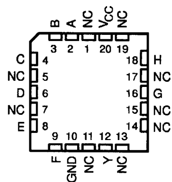
SN54ALS30A, SN54AS30 ... FK PACKAGE (TOP VIEW)
