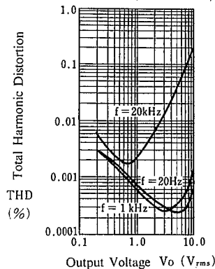
Total Harmonic Distortion vs. Output Voltage
