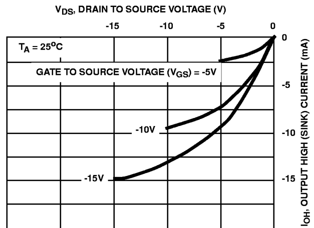
FIGURE 6. MINIMUM OUTPUT HIGH (SOURCE) CURRENT CHARACTERISTICS
