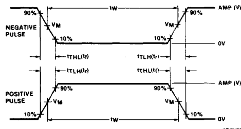
V M = 1.3V for 74LS; V M = 1.5V for all other TTL families.
