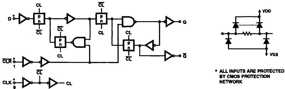
FIGURE 1. 1 OF 4 FLIP-FLOPS
