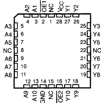
SN54BCT2827C . . . FK PACKAGE (TOP VIEW)
