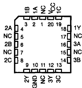
SN54ACT11 ... FK PACKAGE (TOP VIEW)
