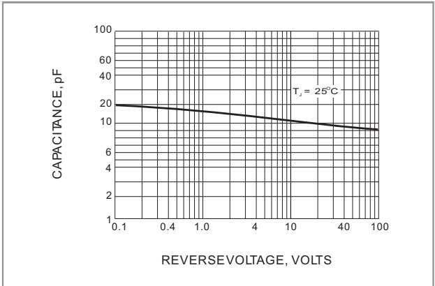
Fig.5-TYPICAL JUNCTION CAPACITANCE
