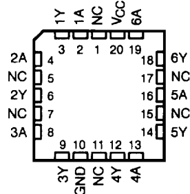
SN54HCT14 . . . FK PACKAGE (TOP VIEW)
