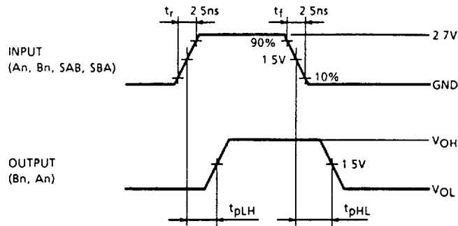
Fig.2 t_{pLH} , t_{pHL}
