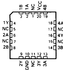
SN54HC03 . . . FK PACKAGE (TOP VIEW)
