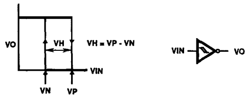
(b) TRANSFER CHARACTERISTIC OF 1 OF 6 GATES
