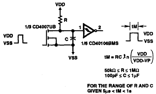
FIGURE 15. MONOSTABLE MULTIVIBRATOR
