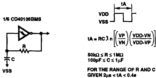
FIGURE 16. ASTABLE MULTIVIBRATOR
