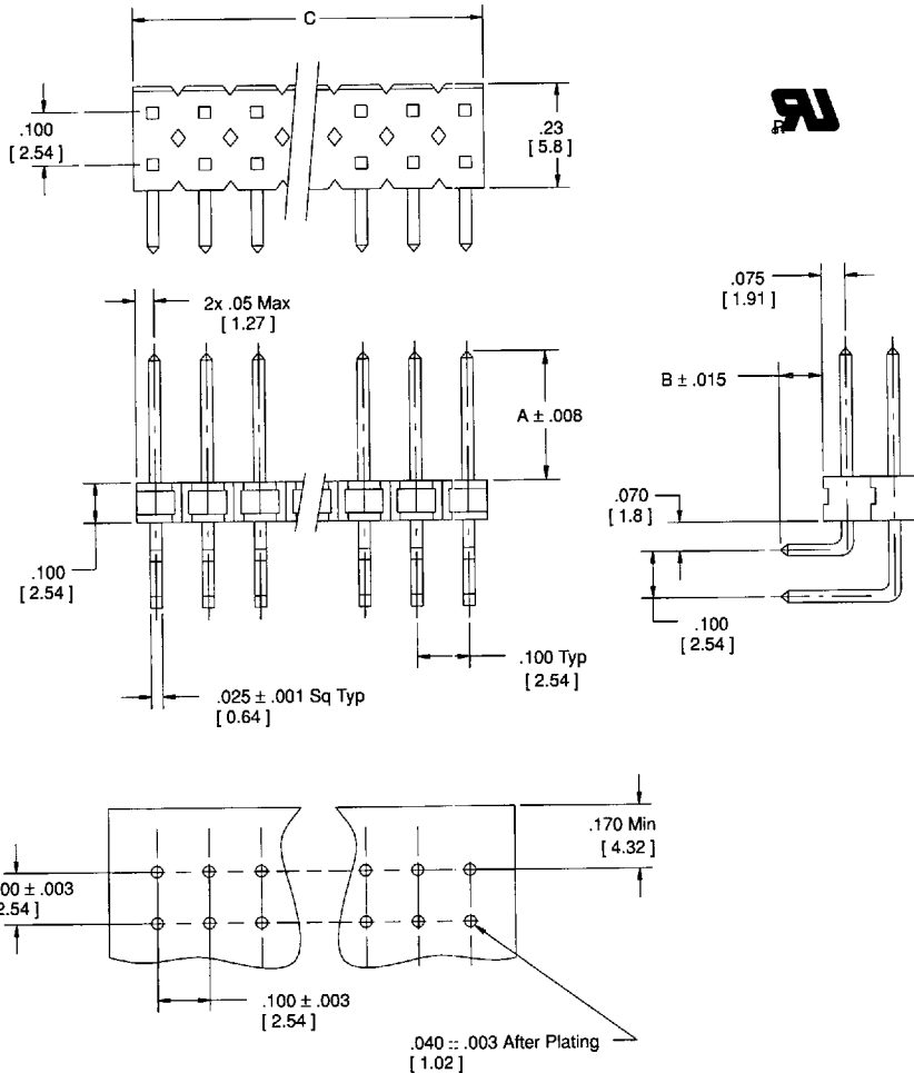
Recommended Hole Pattern
