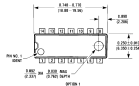
Ceramic Dual-In-Line Package (J) Order Number MM54C901J, MM74C901J, MM54C902J, MM74C902J, MM54C903J, MM74C903J, MM54C904J or MM74C904J NS Package Number J14A
