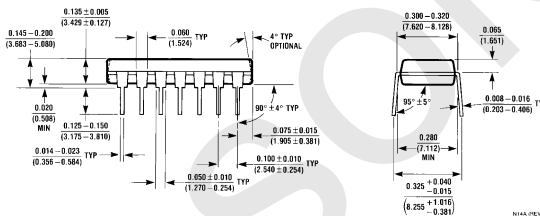
Molded Dual-In-Line Package (N) Order Number MM54C901N, MM74C901N, MM54C902N, MM74C902N, MM54C903N, MM74C903N, MM54C904N or MM74C904N NS Package Number N14A
