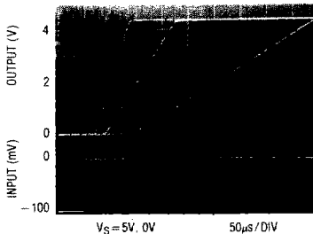
V_S = 5V, 0V 50 \mu s/DIV
