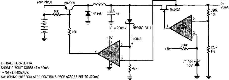
Low Power 9V to 5V Converter
