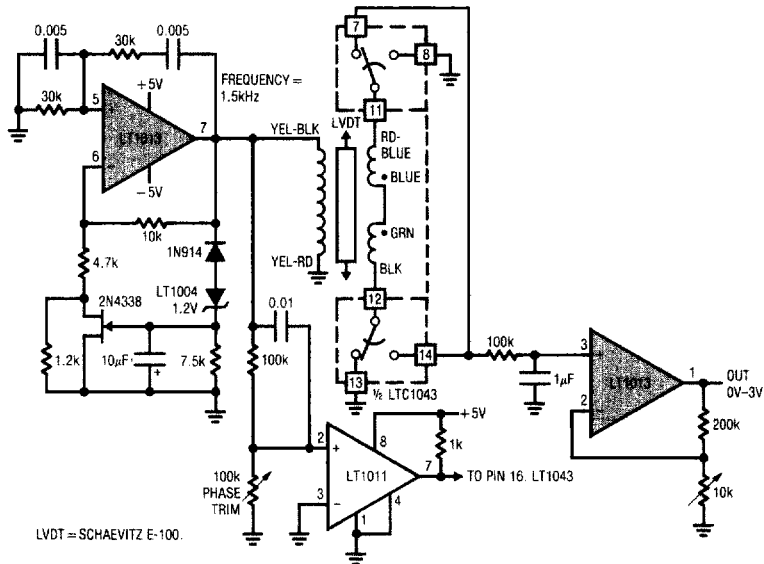
LVDT Signal Conditioner
