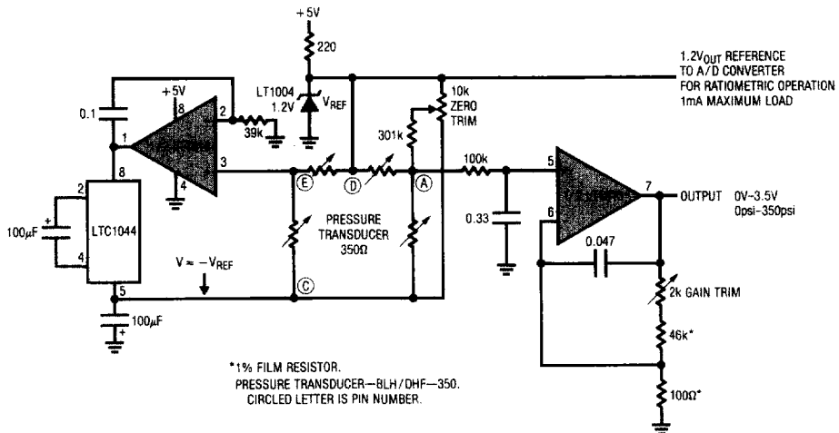
Strain Gage Bridge Signal Conditioner
