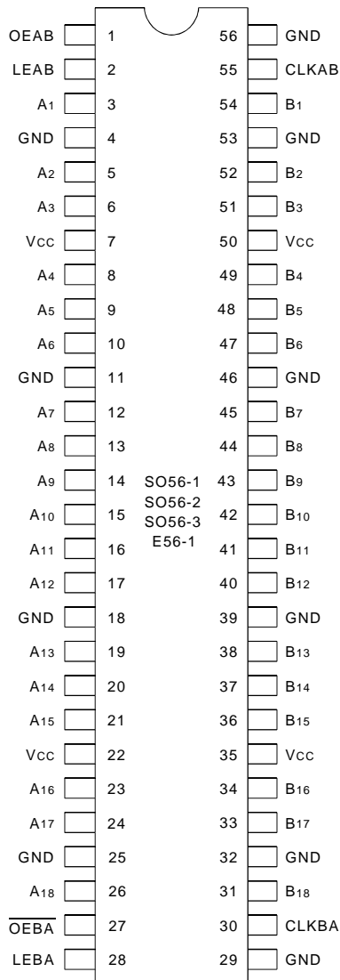
SSOP/ TSSOP/ TVSOP/ CERPACK TOP VIEW
