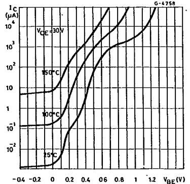
Collector Cutoff Current (NPN types).
