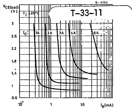
Collector-emitter Saturation Voltage (PNP types).
