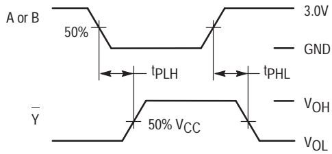
Figure 3. Switching Waveforms
