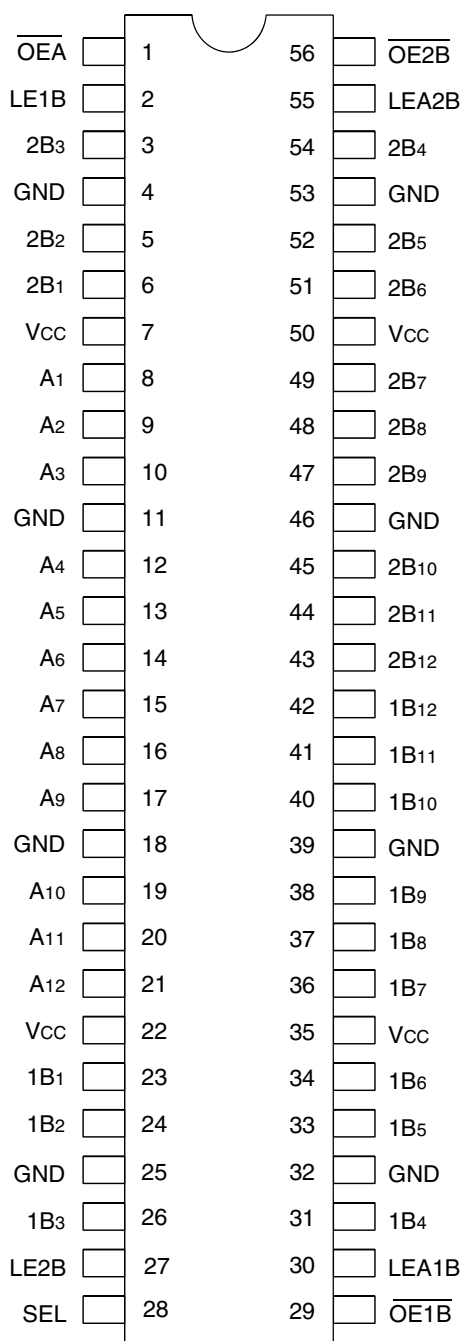
SSOP TOP VIEW
