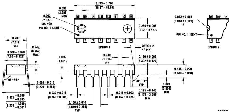
Molded Dual-In-Line Package (N) Order Number LMC13204N, LMC13344N NS Package N16E
