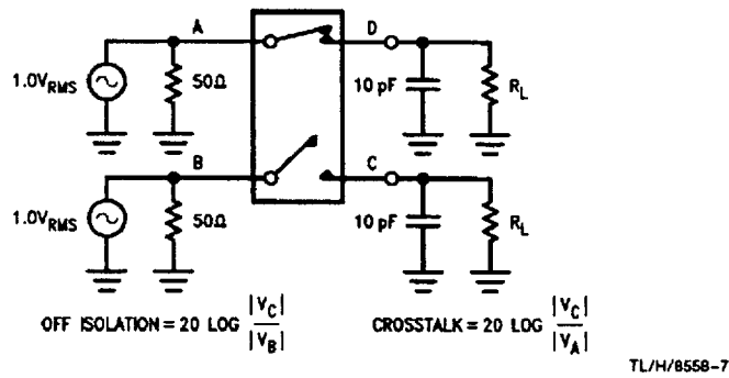
FIGURE 4. "OFF" Isolation, Crosstalk, Small Signal Response
