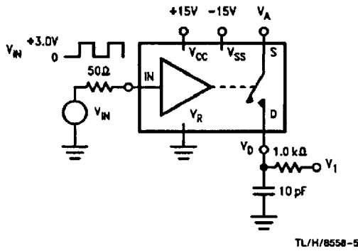
FIGURE 3. t_{ON} , t_{OFF} Test Circuit and Waveforms for a Normally Open Switch
