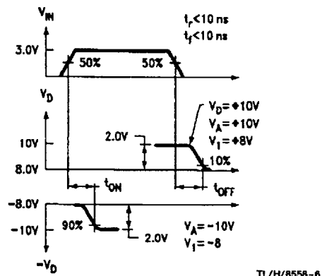
FIGURE 3. t_{ON} , t_{OFF} Test Circuit and Waveforms for a Normally Open Switch
