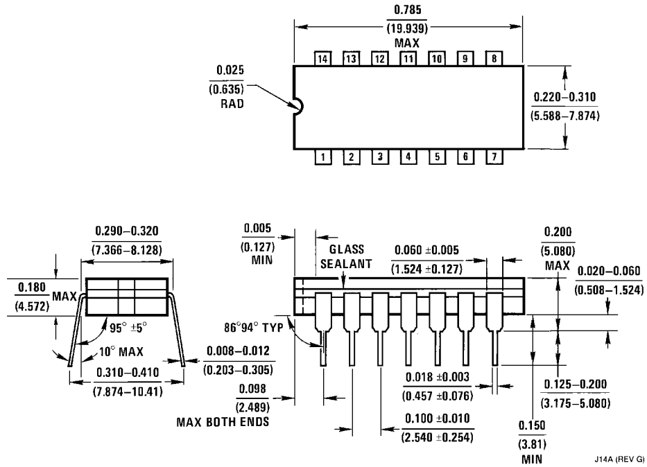
14-Lead Ceramic Dual-In-Line Package (J) Order Number 5486DMQB or DM5486J Package Number J14A
