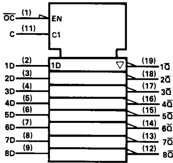
logic symbol†
