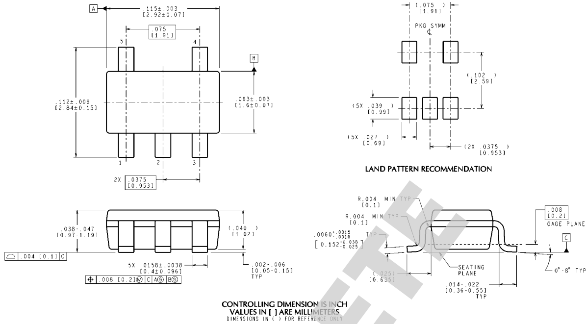
5 Lead Small Outline Package (SOT23-5) NS Package Number MF05A
