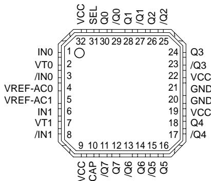
32-Pin MLF™ (MLF-32)
