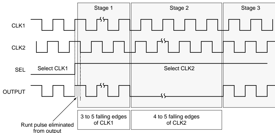
Figure 2. Timing Diagram 1
