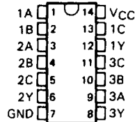
SN54HC11 . . . J PACKAGE SN74HC11 . . . D OR N PACKAGE (TOP VIEW)
