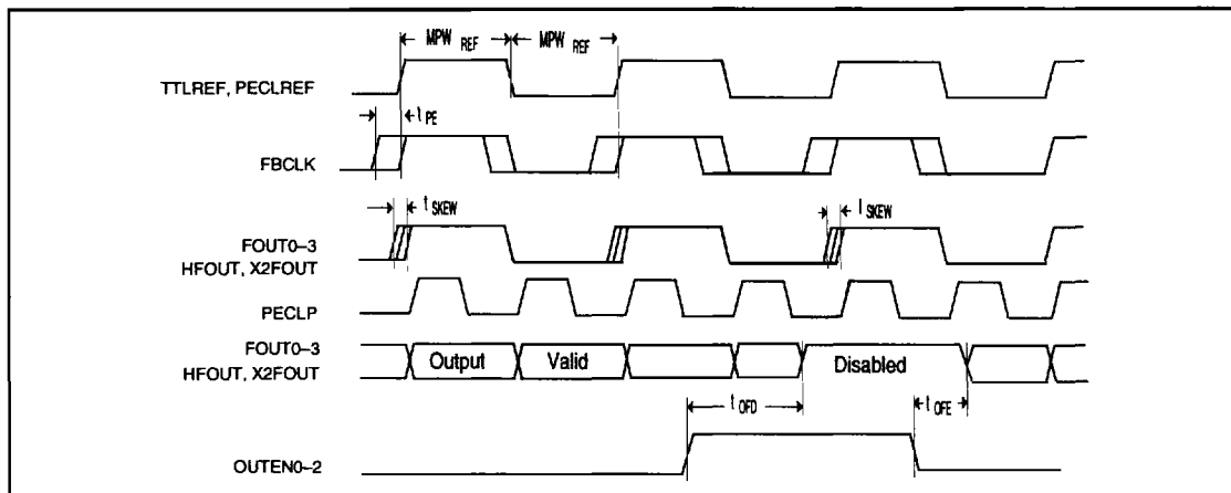
Figure 5. Timing Waveforms
