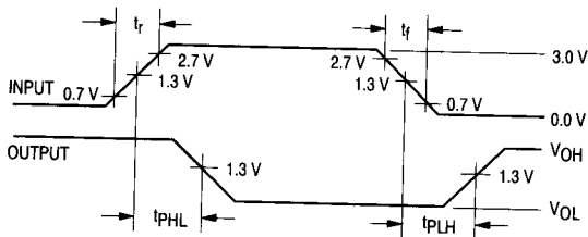
WAVEFORMS
