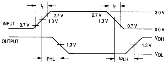
WAVEFORMS
