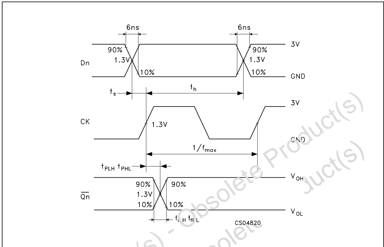
WAVEFORM 1: CK TO \overline{Qn} PROPAGATION DELAYS, CK MAXIMUM FREQUENCY, Dn TO CK SETUP AND HOLD TIMES ( f=1\text{MHz} ; 50% duty cycle)
