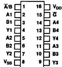
16-Lead Flatpack Top View
