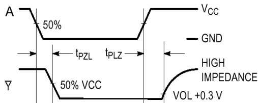
Figure 5. Switching Waveforms
