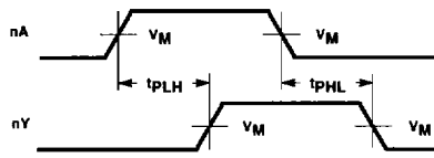
Waveform 1. Propagation Delay For Input to Output
