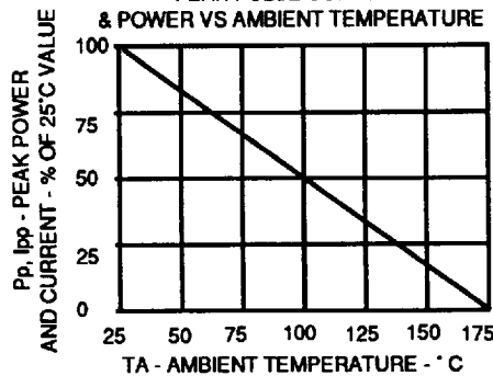
FIG 3 MAXIMUM ALLOWABLE PEAK PULSE CURRENT & POWER VS AMBIENT TEMPERATURE
