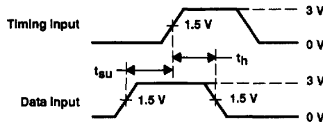
VOLTAGE WAVEFORMS
